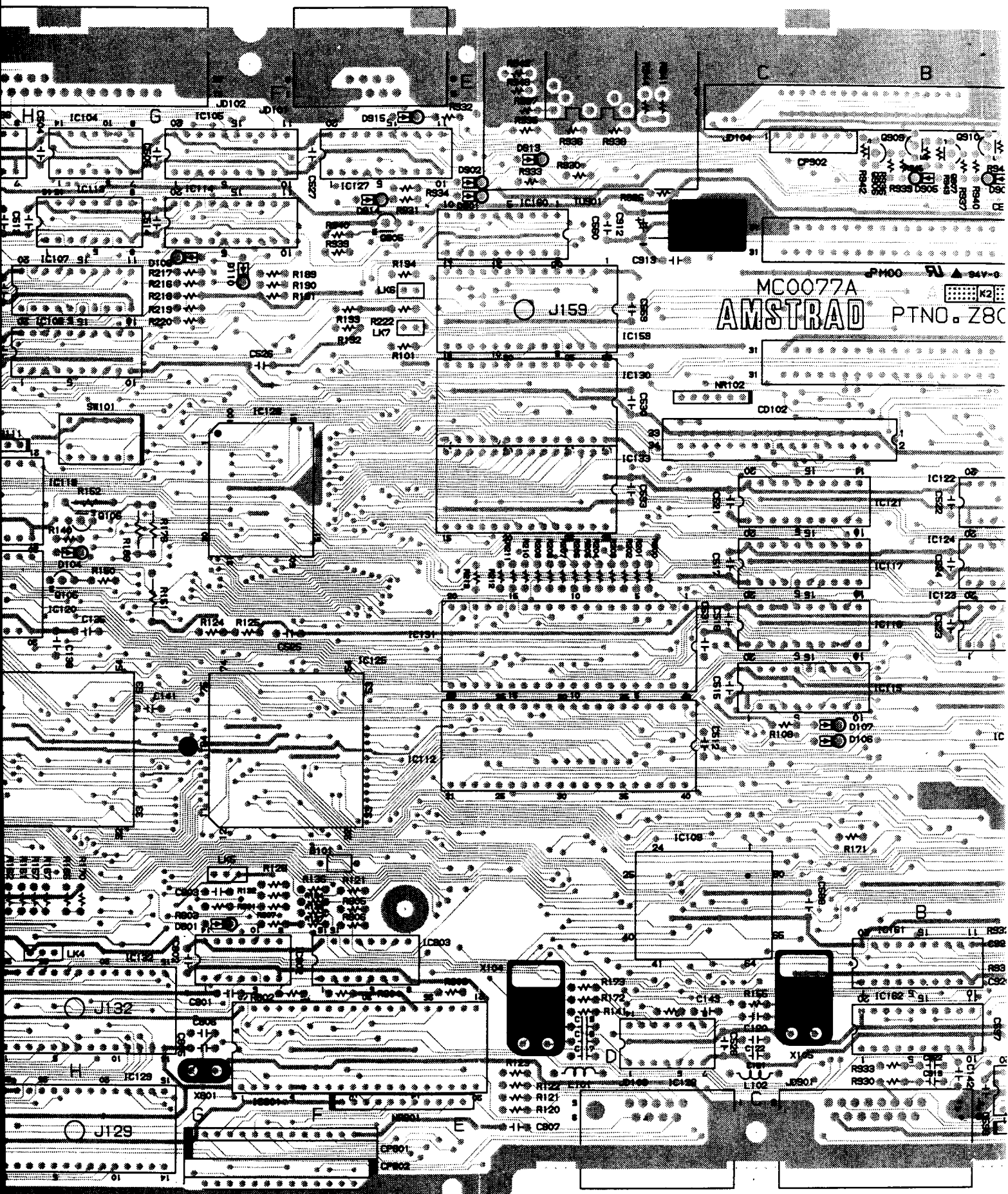
MAIN PCB (TOP VIEW)
