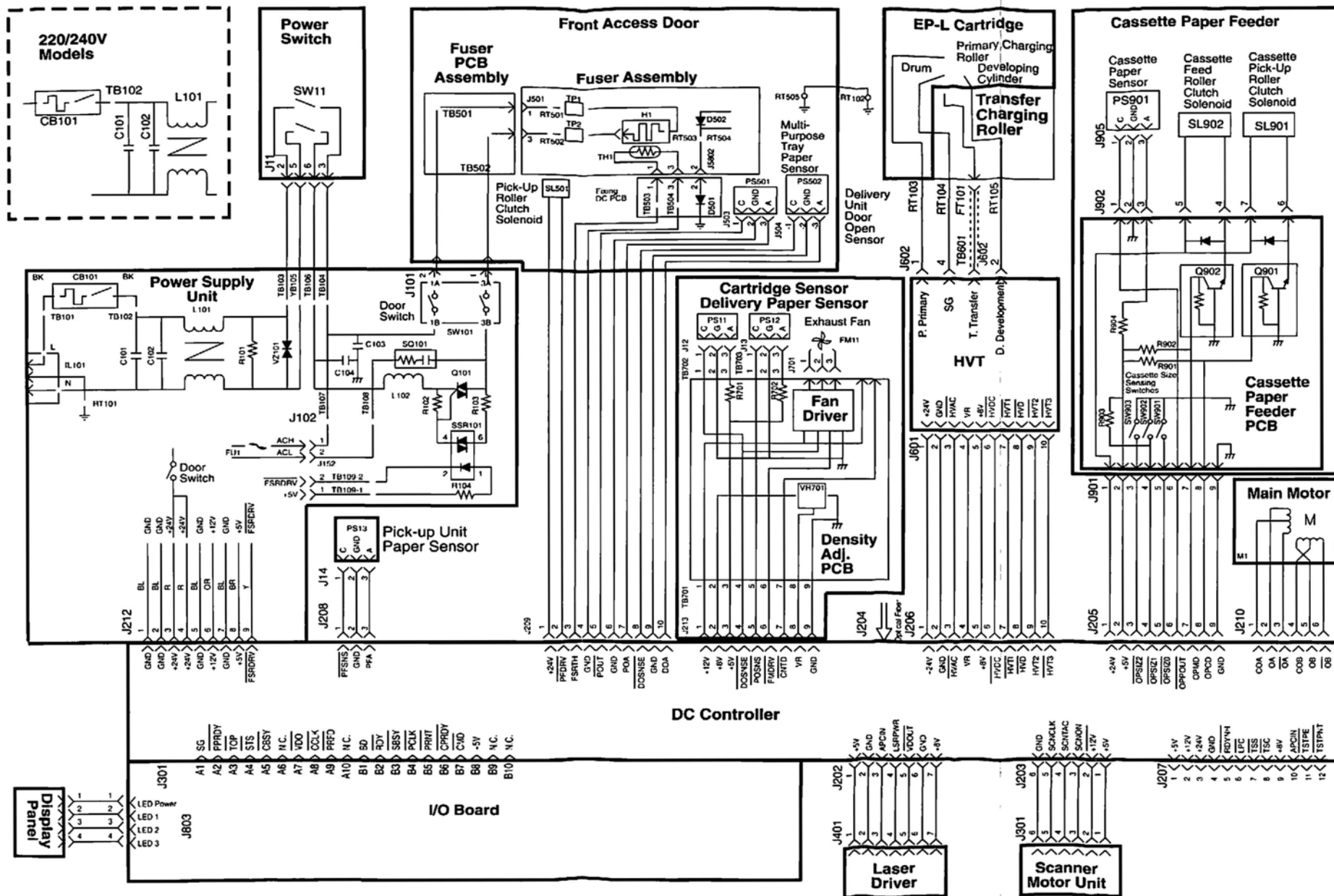
Personal LaserWriter LS Wiring Diagram
