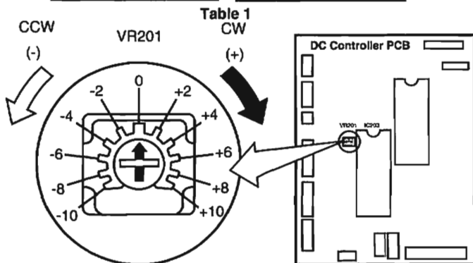
Figure: VR201 Adjustment Settings
