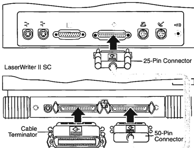
Figure: SCSI Connection
