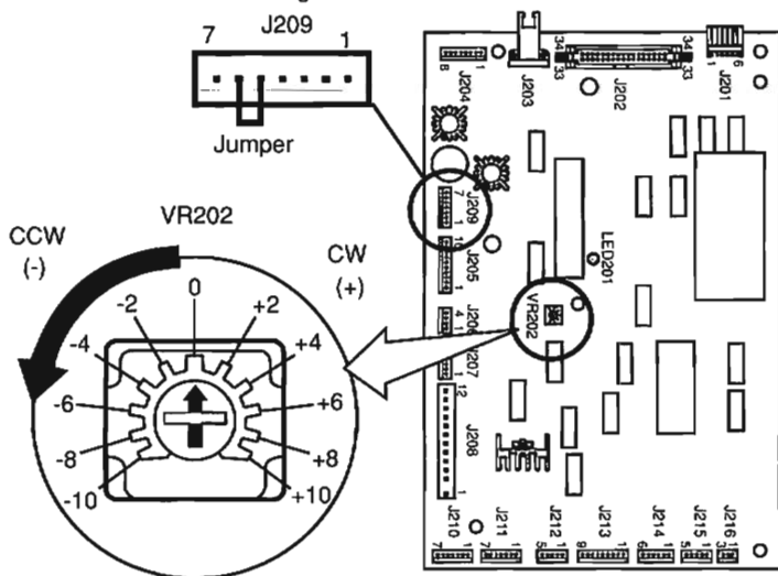
Figure: DC Controller PCB
