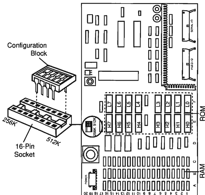
Figure: LaserWriter 256K/512K I/O Board
