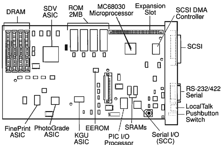
Figure: Ilg Controller-I/O Board
