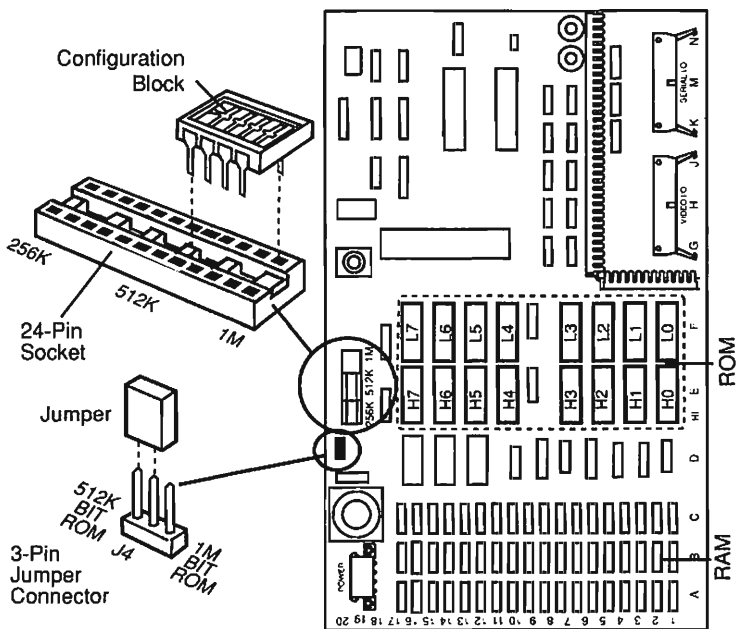
Figure: LaserWriter 512K/1M I/O Board
