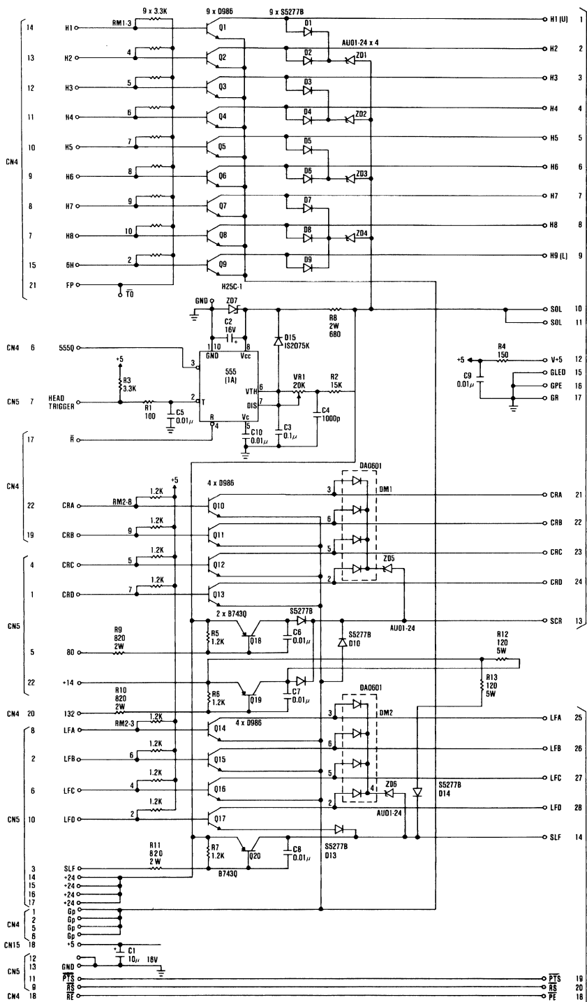
Graphics Printer Driver Circuit
