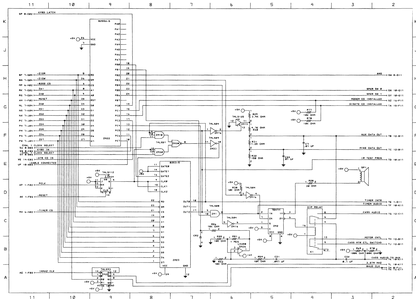
System Board (Sheet 9 of 17)
