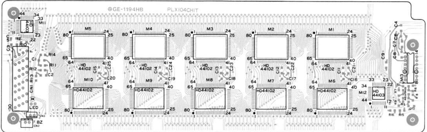
(TOP VIEW)
