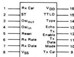
Fig. C-21 MC14412 Pin Layout
