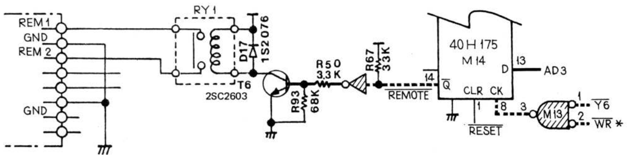
Fig. 4-10 Remote Circuit of Cassette Interface
