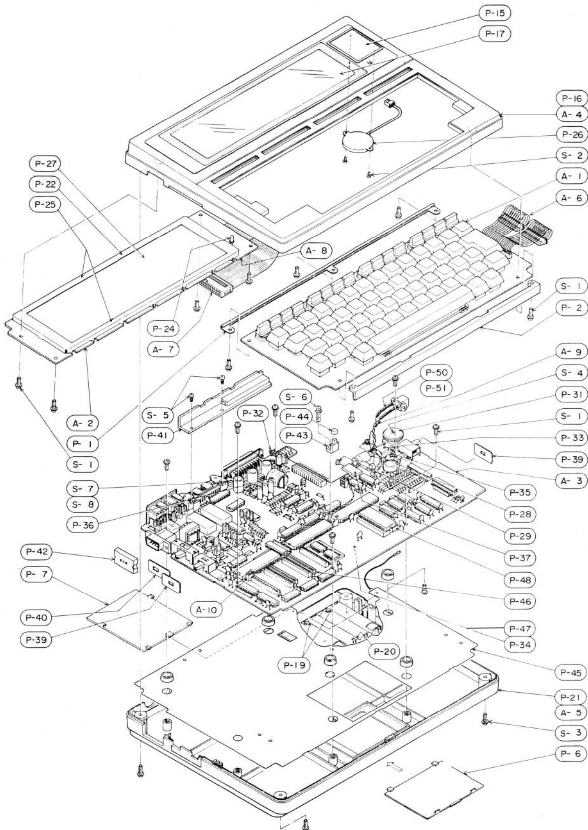
Fig. 6-1 Exploded View
