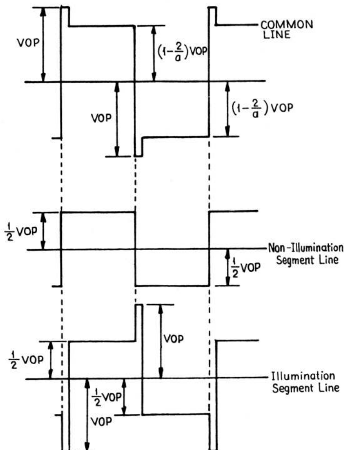
Fig. 4-36 LCD Waveform
