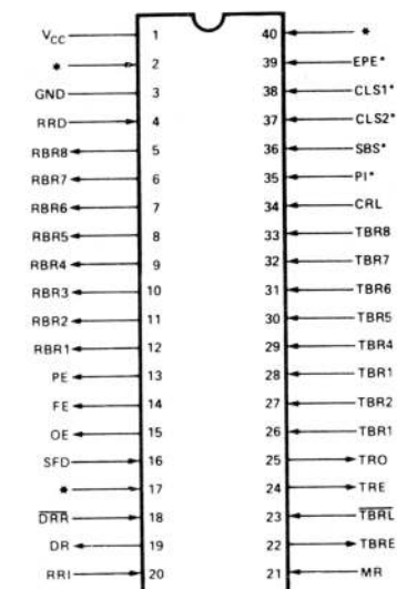
Fig. C-14 IM6402 Pin Layout
