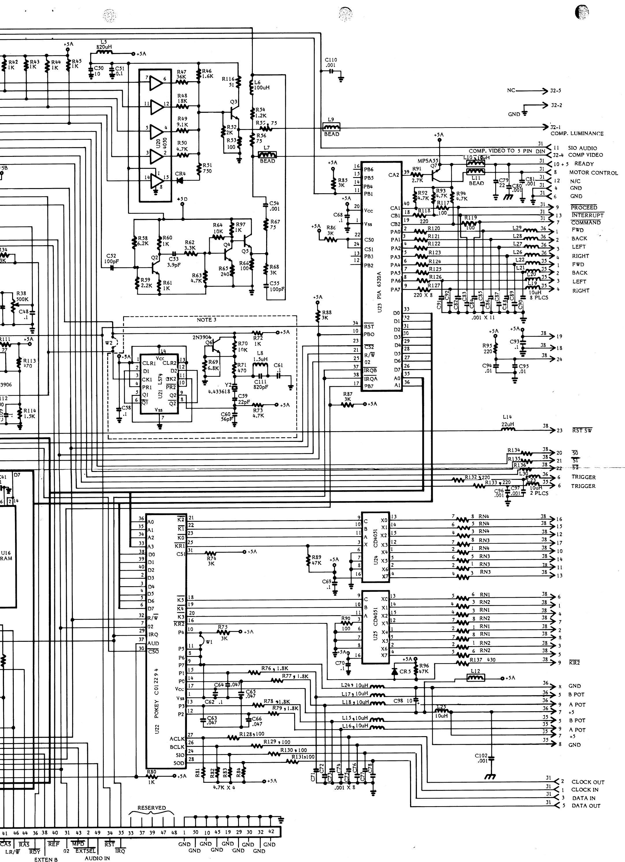
800 XL SCHEMATIC
