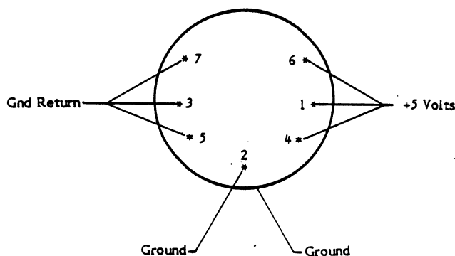
Figure 1-8. Power Supply Pin Assignments (Looking Toward Computer)
