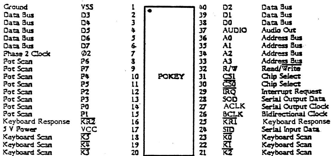
Figure 1-6. POKEY pin assignments
